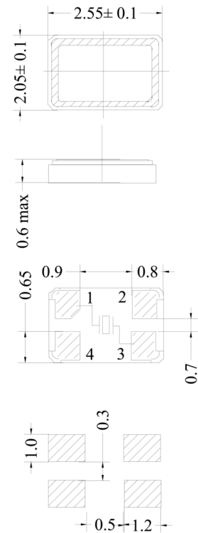
Recommended Land Pattern
