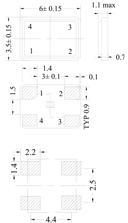
Recommended Solder Pad Layout
